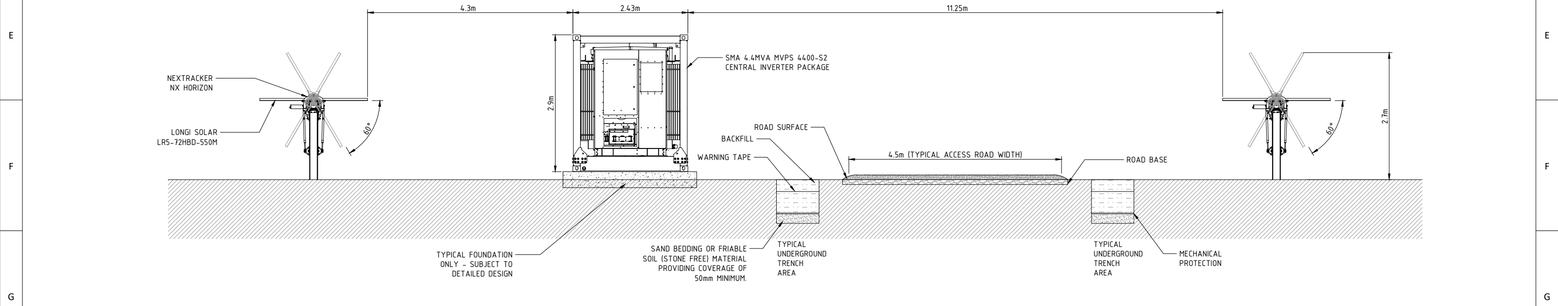
TYPICAL ACCESS ROAD AND INVERTER STATION SECTION VIEW
